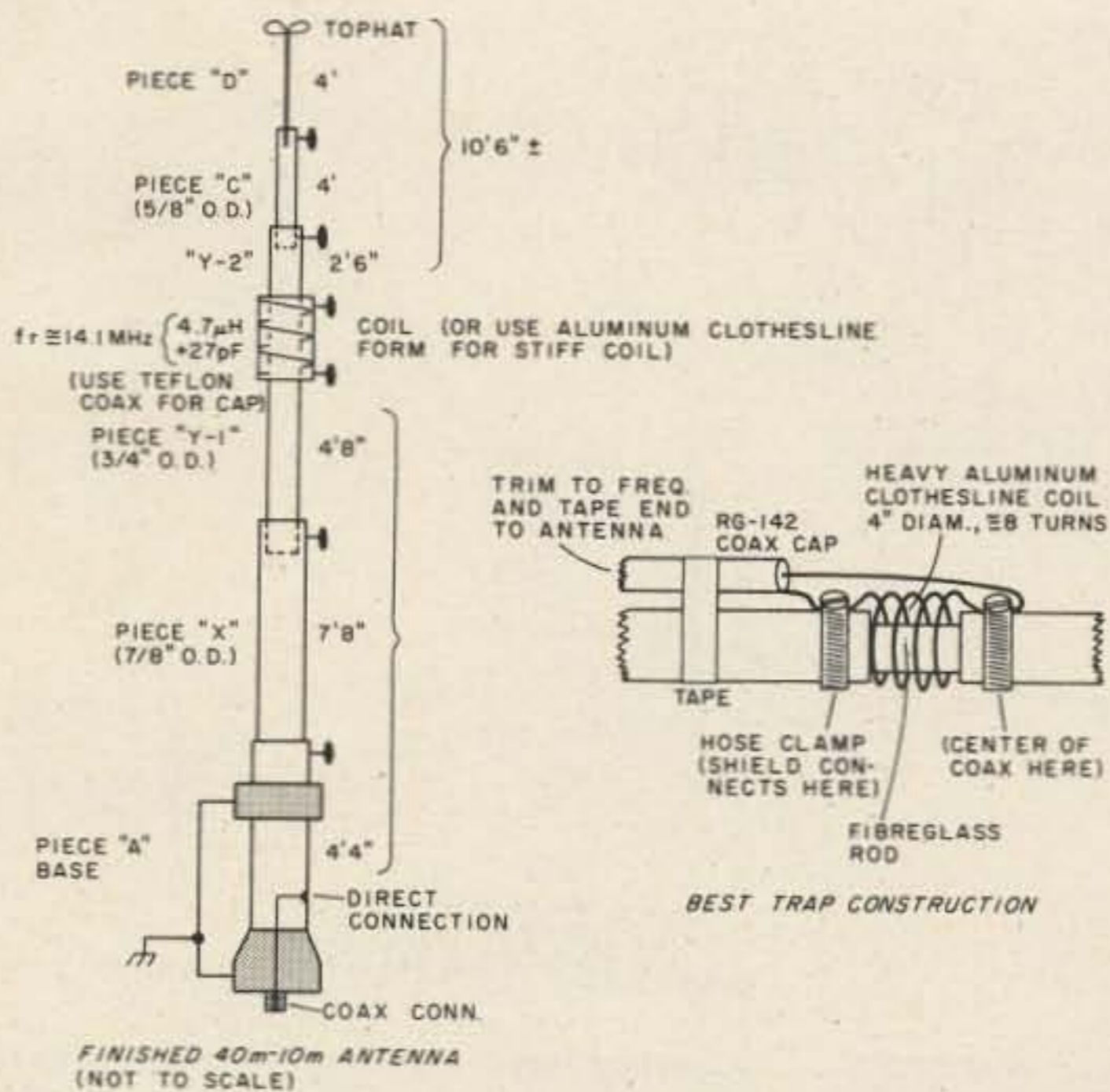
Fig. 4. Variant C - 10 to 40 meter trap vertical.
