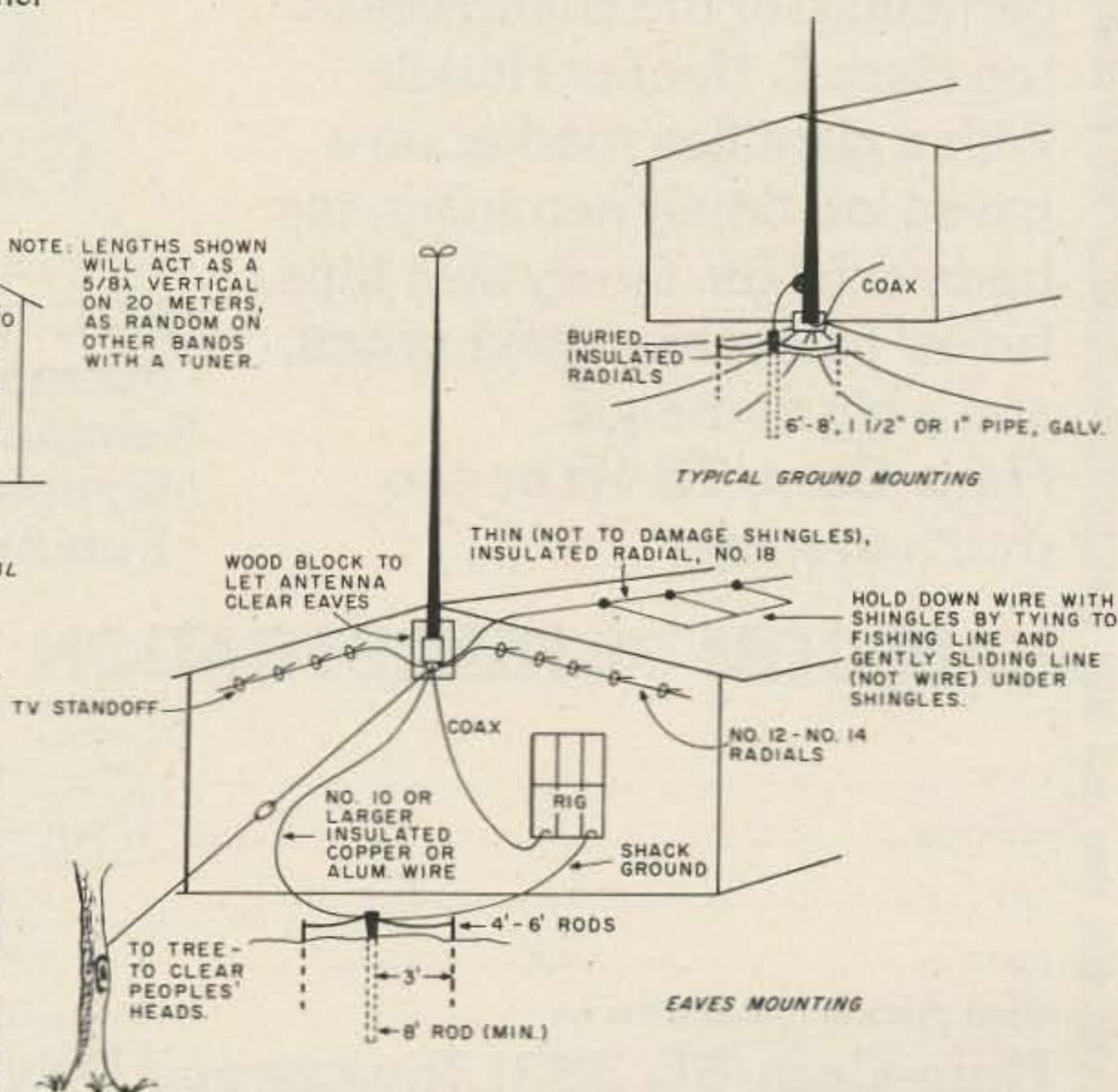
Fig. 6. Installation suggestions.
