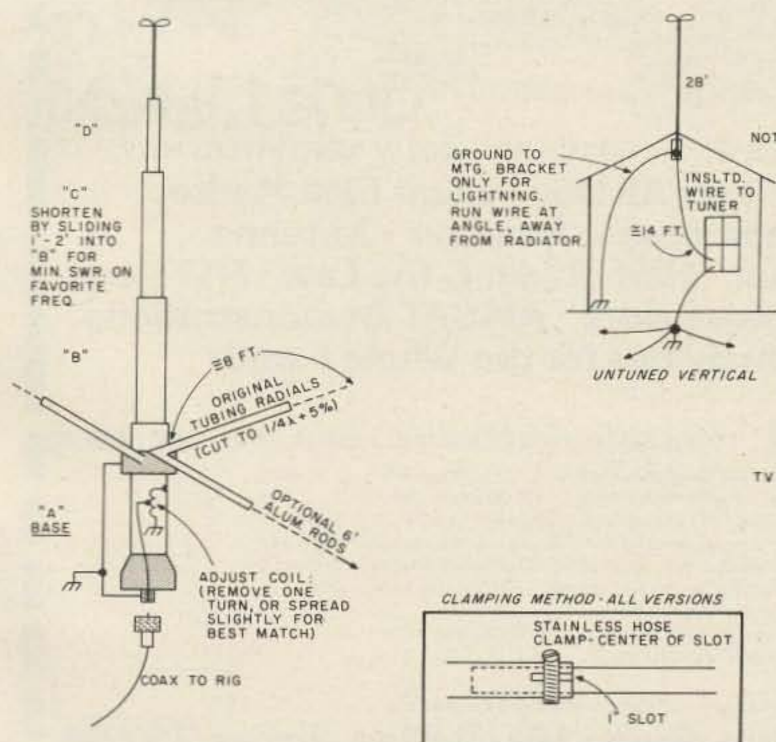
Fig. 5. Variant D - 10 meter \frac{1}{2}\lambda vertical.
